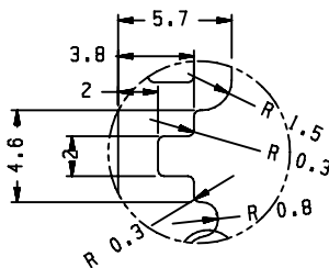
DETAIL K SCALE 7/2
